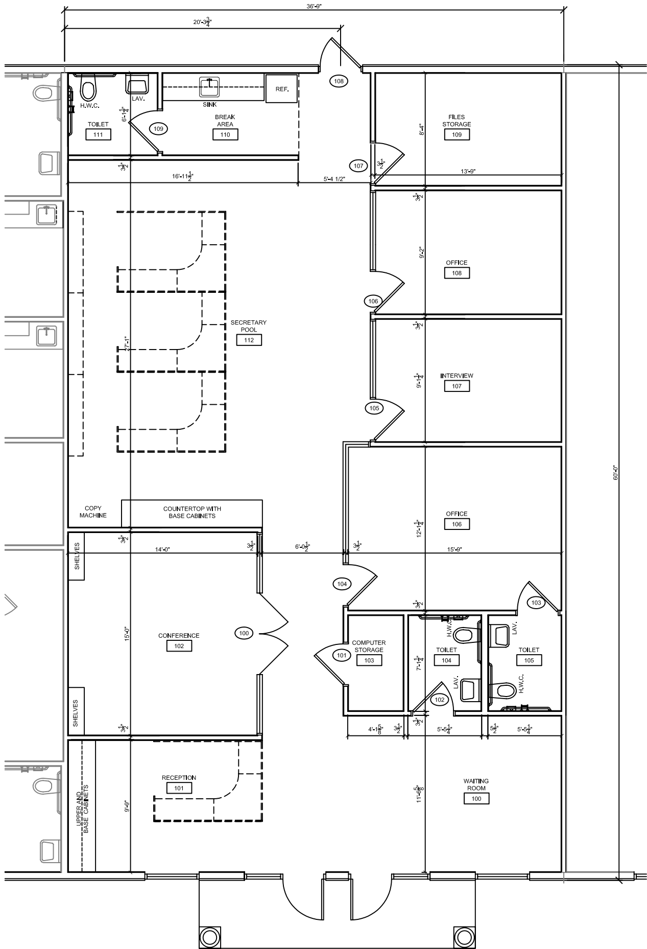
01 Plan - Holman Law Office Scale: 1/4" = 1'-0"
